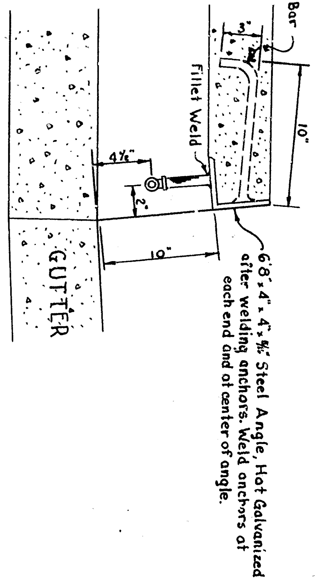
SECTION OF OUTLET NO SCALE
