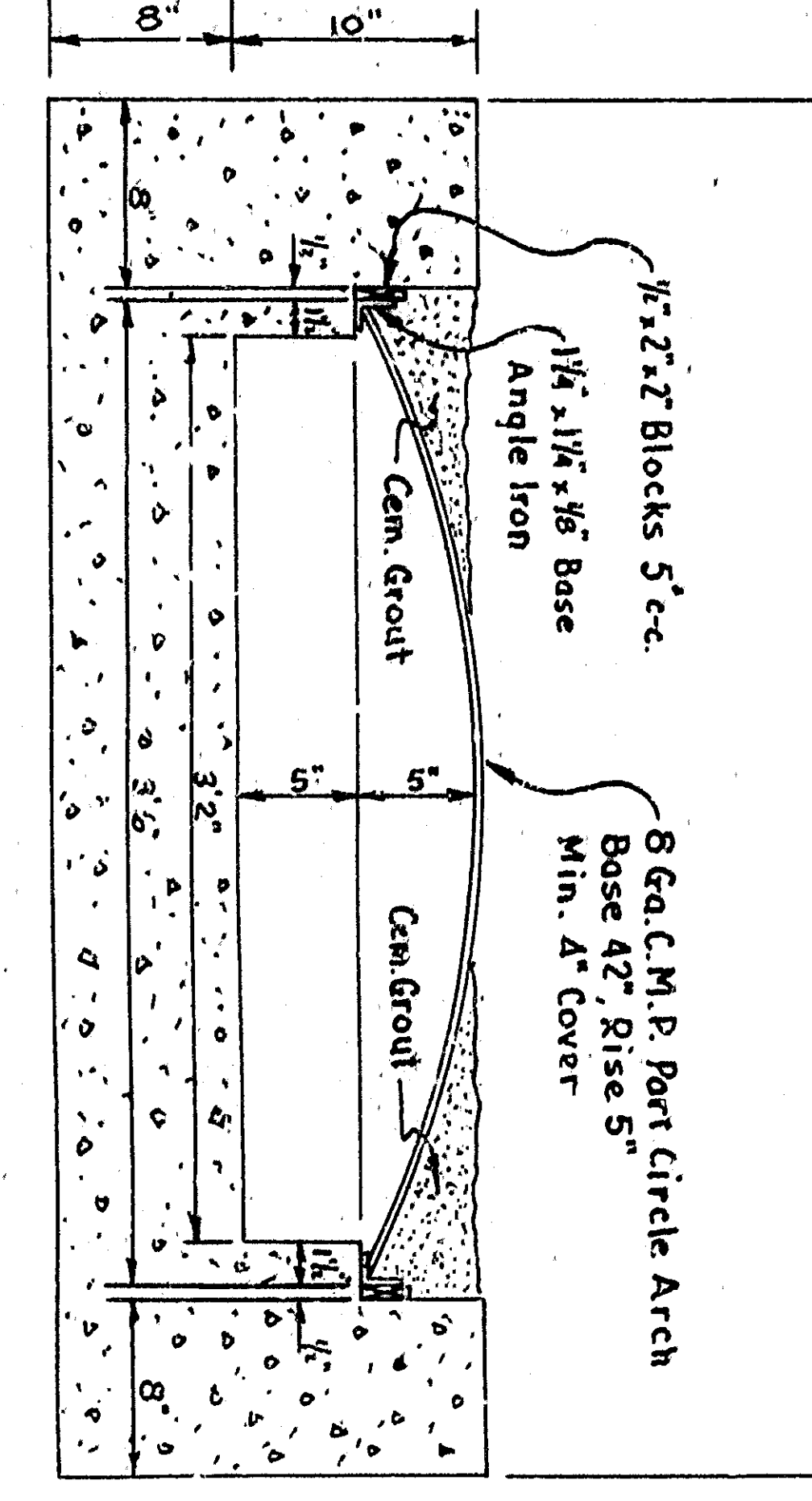
SECTION OF PART CIRCLE CULVERT SCALE 1"-1'
