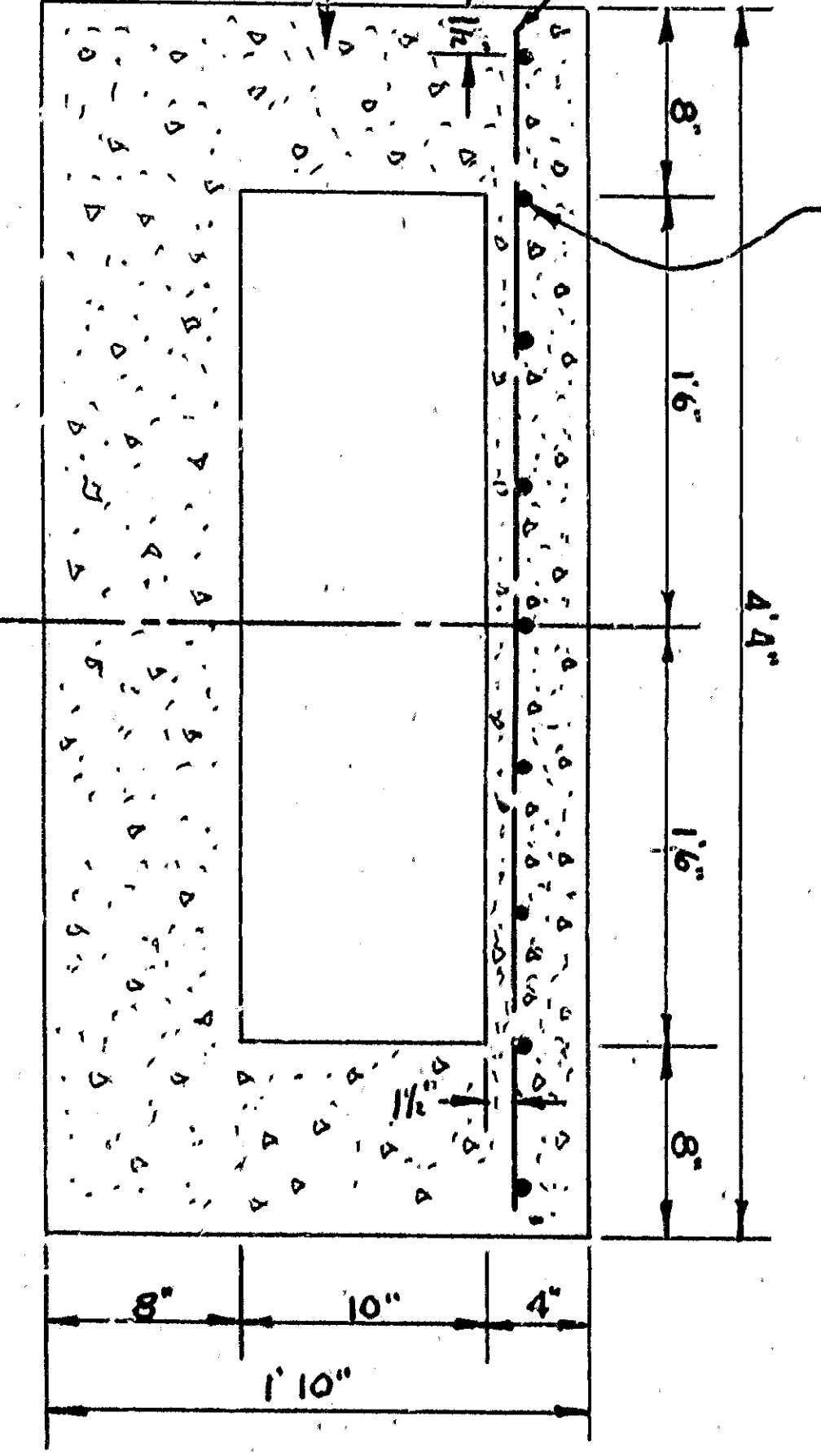
SECTION OF REINFC CONC BOX SCALE 1"-1'
